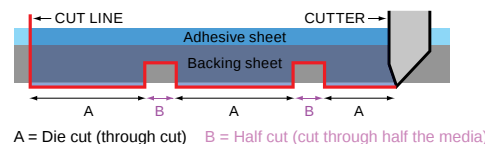
The half cut function is Mimaki's proprietary technology
